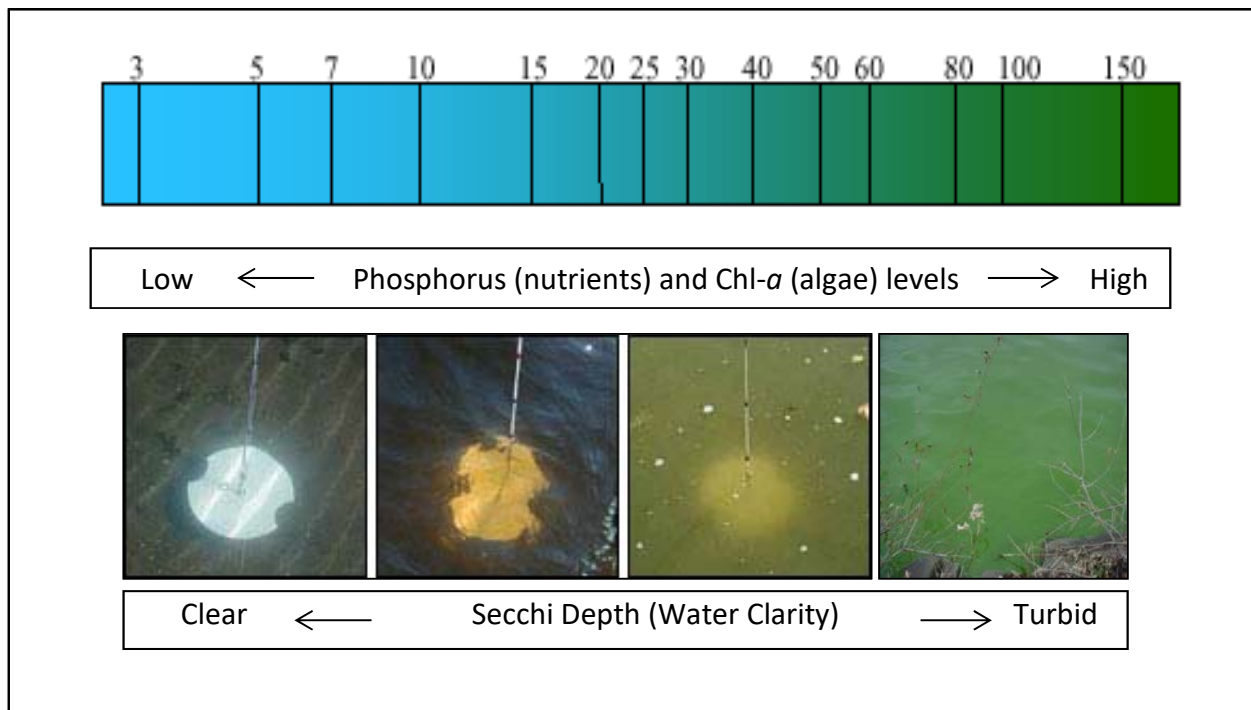
Figure 6. Relationships between lake phosphorus and algae levels with water clarity (WCD)
